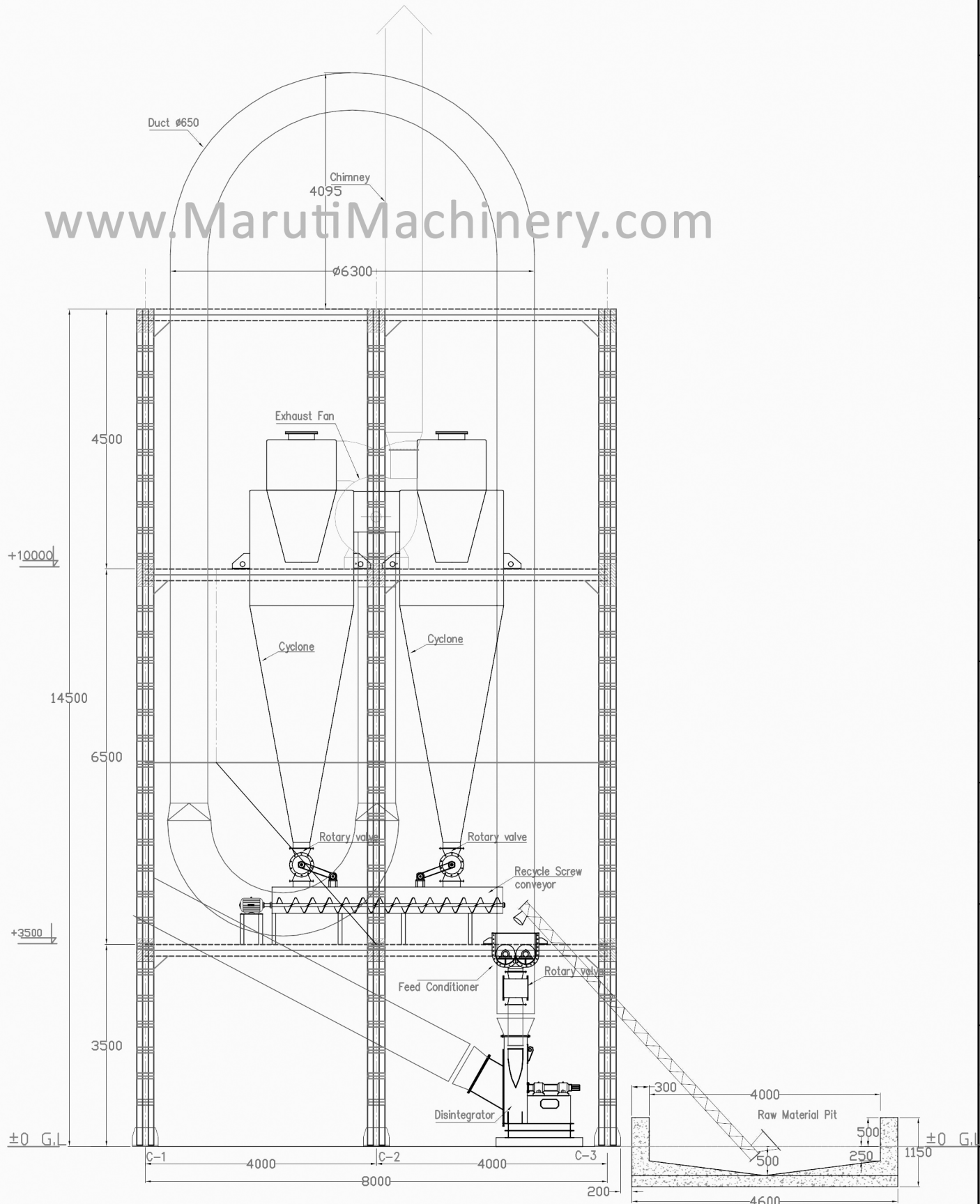
FRONT VIEW OF GLUTEN DRYER
